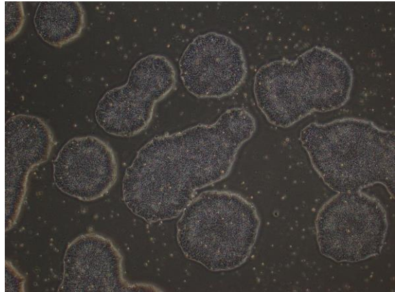
CiRA-j-1595-D: passage-3
